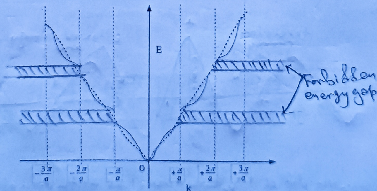
Fig: Dispersion relation for the electron moving in parabolic periodic lattice.
